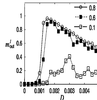
FIG. 5. The output overlap m_{\text{out}}^1 against the fluctuation intensity D for m_{\text{in}}^1=0.8, 0.6 , and 0.1 with N=200 , p=3 , and a=0.5 . Stochastic resonancelike phenomenon is observed for m_{\text{in}}^1=0.8 and 0.6 .
