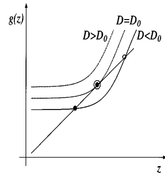
FIG. 8. Schematic diagram of bifurcation of g(z) .
