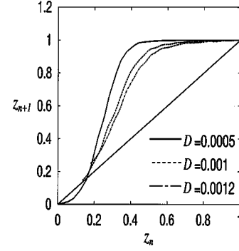
FIG. 7. Numerically obtained g(z_n) for D=0.0005 , 0.001 , and 0.0012 with N=100 and I=0.1 . A saddle-node bifurcation at D \sim 0.001 is observed.
