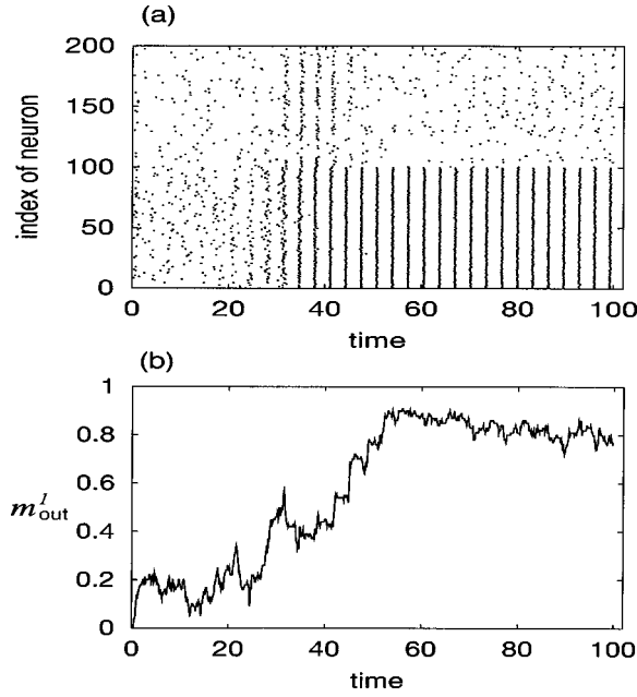
FIG. 3. The result of numerical simulation. (a) The firing times of all the neurons and (b) the output overlap m_{\text{out}}^1 with the pattern \xi^1 , for N=200 , p=3 , a=0.5 , and D=0.002 . The retrieval of the pattern \xi^1 is successful.
