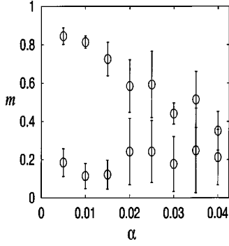
FIG. 6. The basin of attraction for N=200 , D=0.002 , and a=0.5 . The error bar denotes the standard deviation for ten samples. The storage capacity is estimated to be about 0.02.
