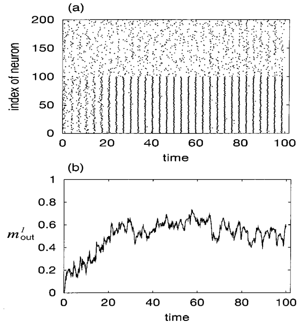
FIG. 4. The result of numerical simulation. (a) The firing times of all the neurons and (b) the output overlap m_{\text{out}}^1 with the pattern \xi^1 , for N=200 , p=3 , a=0.5 , and D=0.004 . The neurons which store 0's for pattern \xi^1 fire with high firing rates due to the large fluctuation intensity, so the output overlap is lower than the case of D=0.002 .
