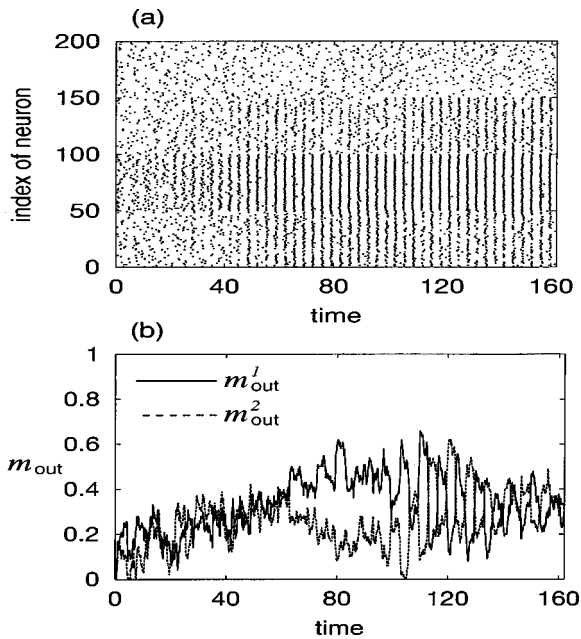
FIG. 11. The results of numerical simulation. (a) The firing times and (b) the output overlaps, for N=200 , p=3 , a=0.5 , D=0.004 , and d_p=6.5 . All the neurons are firing with high firing rates, so the retrievals of both pattern \xi^1 and pattern \xi^2 fail.
