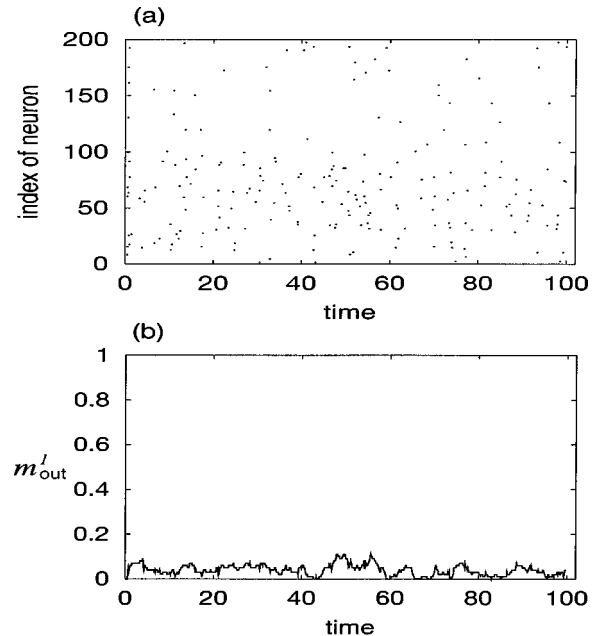
FIG. 2. The result of numerical simulation. (a) The firing times of all the neurons and (b) the output overlap m_{out}^1 with the pattern \xi^1 , for N=200 , p=3 , a=0.5 , and D=0.001 . All the neurons are firing randomly, so the retrieval of the pattern \xi^1 fails.
