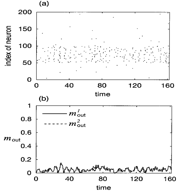
FIG. 9. The results of numerical simulation. (a) The firing times and (b) the output overlaps, for N=200 , p=3 , a=0.5 , D=0.001 , and d_p=6.5 . The retrievals of both pattern \xi^1 and pattern \xi^2 fail.
