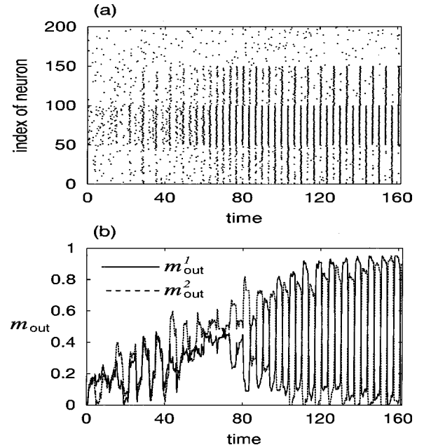
FIG. 10. The results of numerical simulation. (a) The firing times and (b) the output overlaps, for N=200 , p=3 , a=0.5 , D=0.002 , and d_p=6.5 . The alternate retrieval of two patterns is observed as the antiphase oscillations of two output overlaps.
