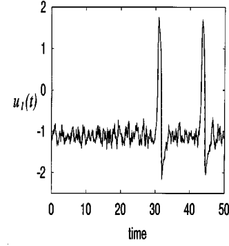
FIG. 1. A typical time series of u_1(t) for N=200 , p=3 , a=0.5 , and D=0.001 . The fluctuation around u_{eq} and the two firings are observed.
